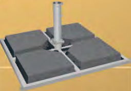
METAL CROSS BASE 1160 x 1160 / Ø 78
